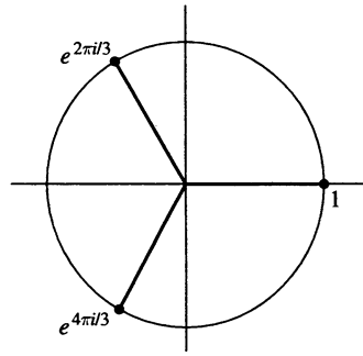
cube roots of unity
