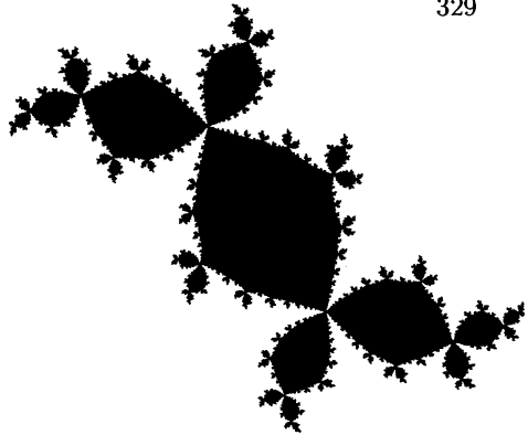
Douady's rabbit ( c \approx -0.122 + 0.745i )
