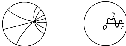
hyperbolic geodesics
