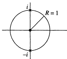
singularities at \pm i
