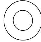
not star-shaped
