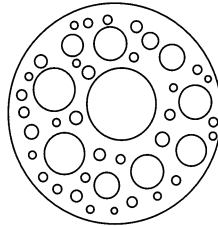
Swiss cheese set
