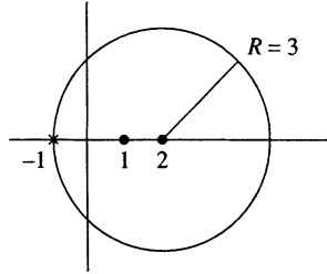
singularity at -1 , analytic at +1
