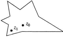
star-shaped with respect to z_0 but not z_1
