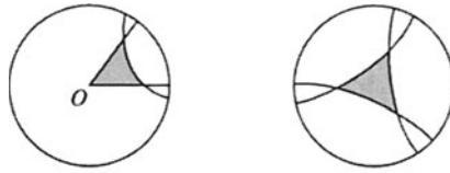
hyperbolic triangles
