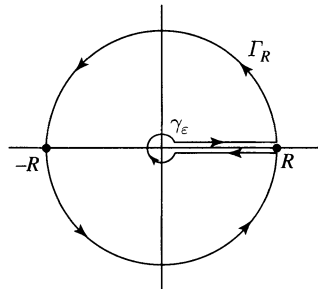
keyhole contour
