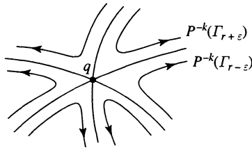
critical point of order m = 2
