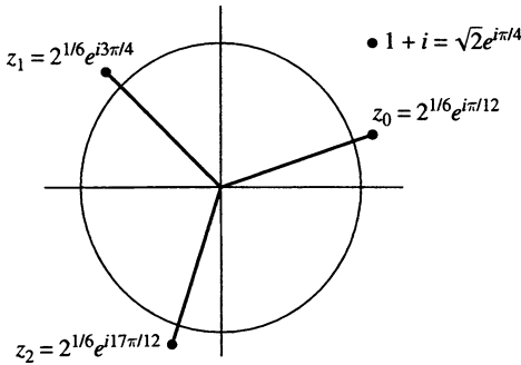
cube roots of 1 + i
